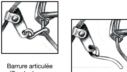
S-Hook + J-Hook
